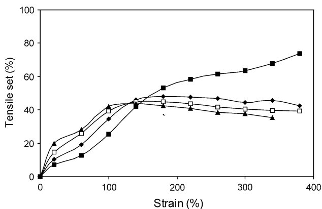
Fig. 8 The TS as a function of strain as determined by a cyclic staircase TS test and the TS values calculated from the strain increment for PTMO 2000 -T6A6T at four temperatures; ■, 20 °C; ◆, 50 °C; □, 80 °C; ▲, 110 °C
